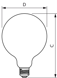
MASTER VLE LEDBulb D5.9-60W E27 927 G120CLG
