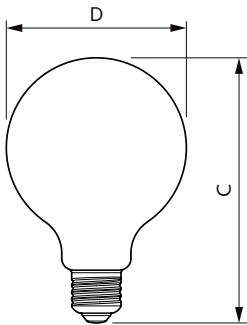
G93 230V 9-60W 806lm 2700-2200K E27 D CL
